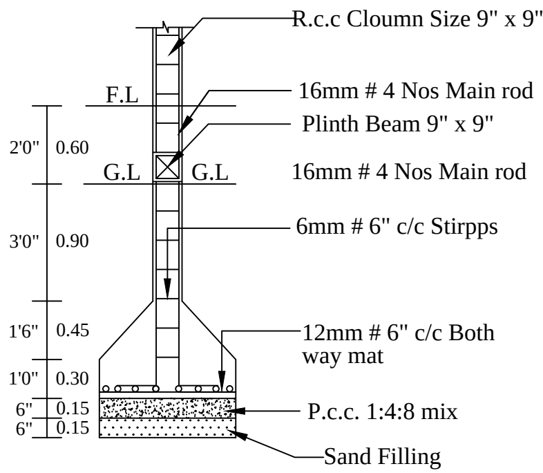
COLUMN DETIALS
