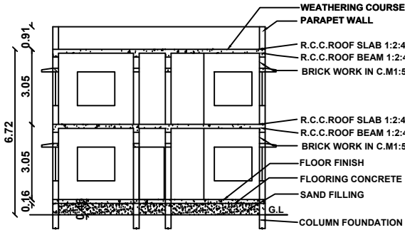
SECTION ON GG
