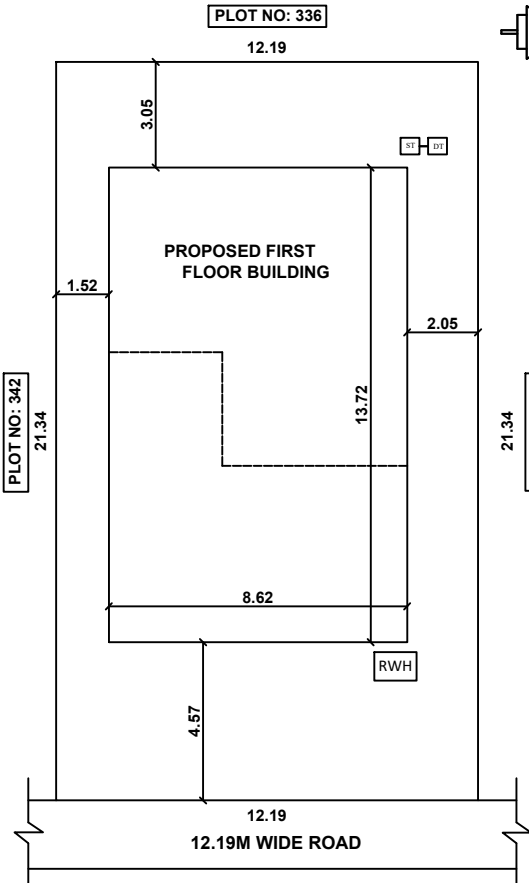
SITE PLAN
