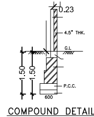
COMPOUND DETAIL
