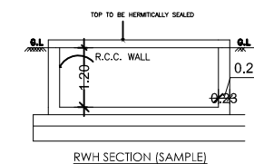
RWH_CAPACITY_L=2000LTRS
