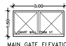
MAIN GATE ELEVATION
