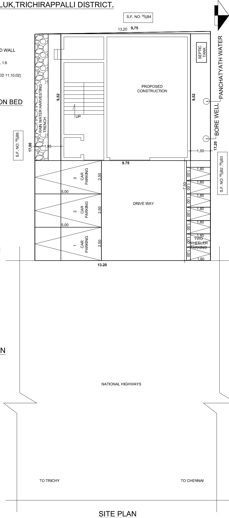
SITE PLAN
