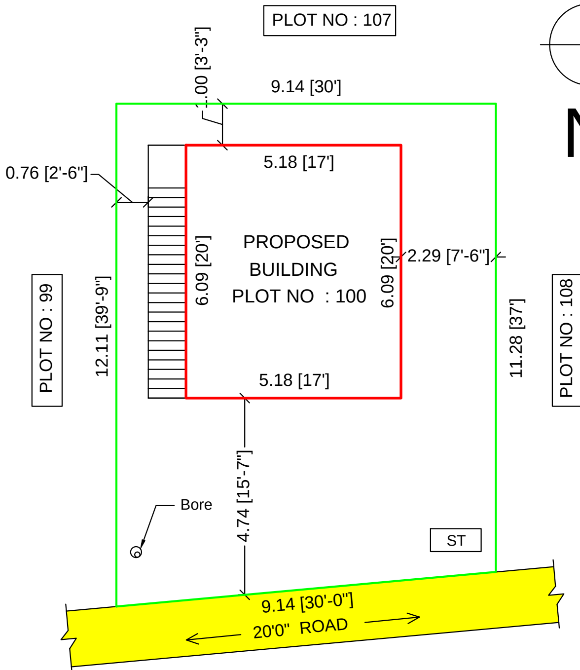
SITE PLAN
