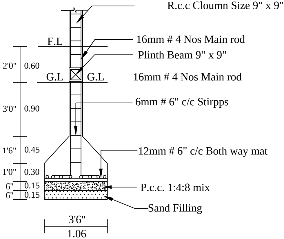
COLUMN DETAILS
