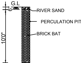
PERCOLATION PIT
