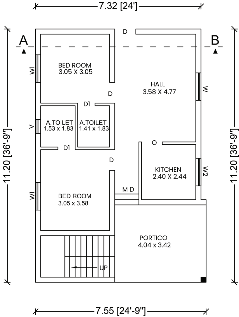
PLAN
