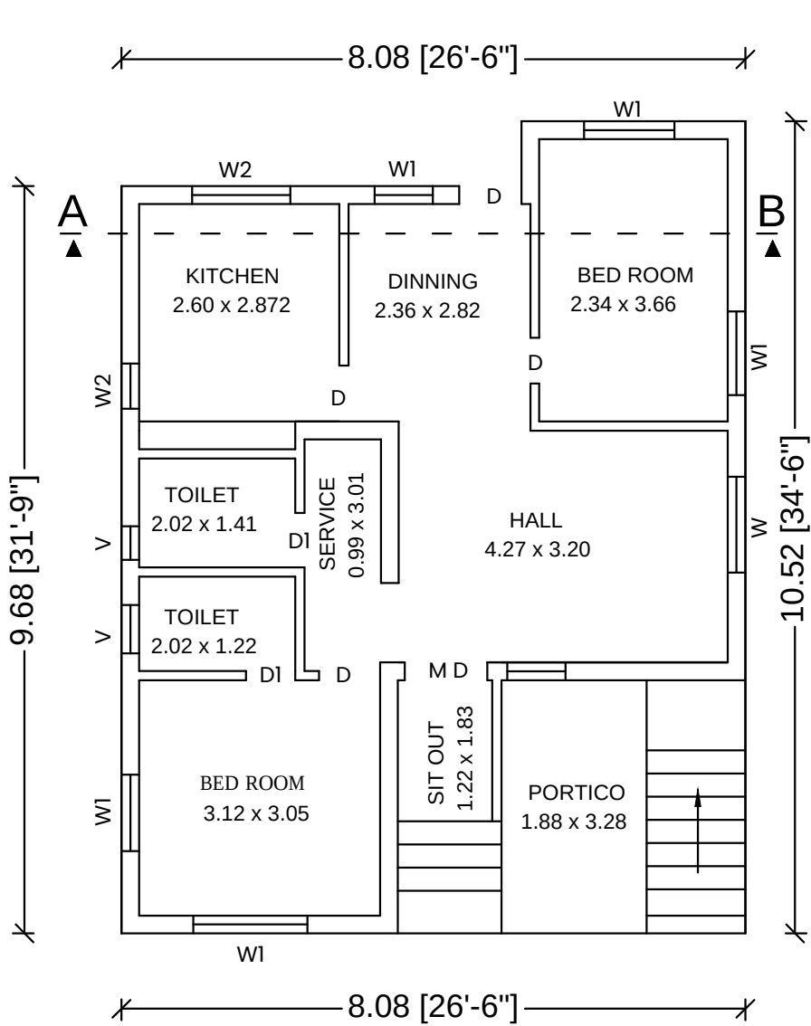
PLAN
