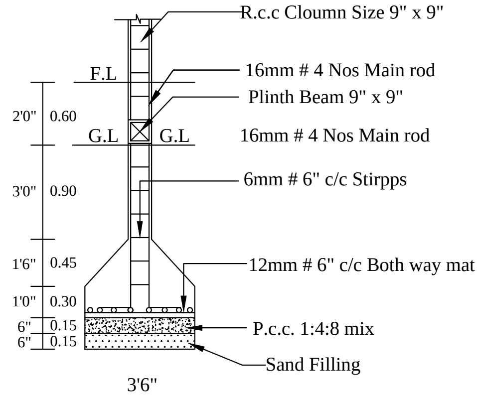
COLUMN DETIALS
