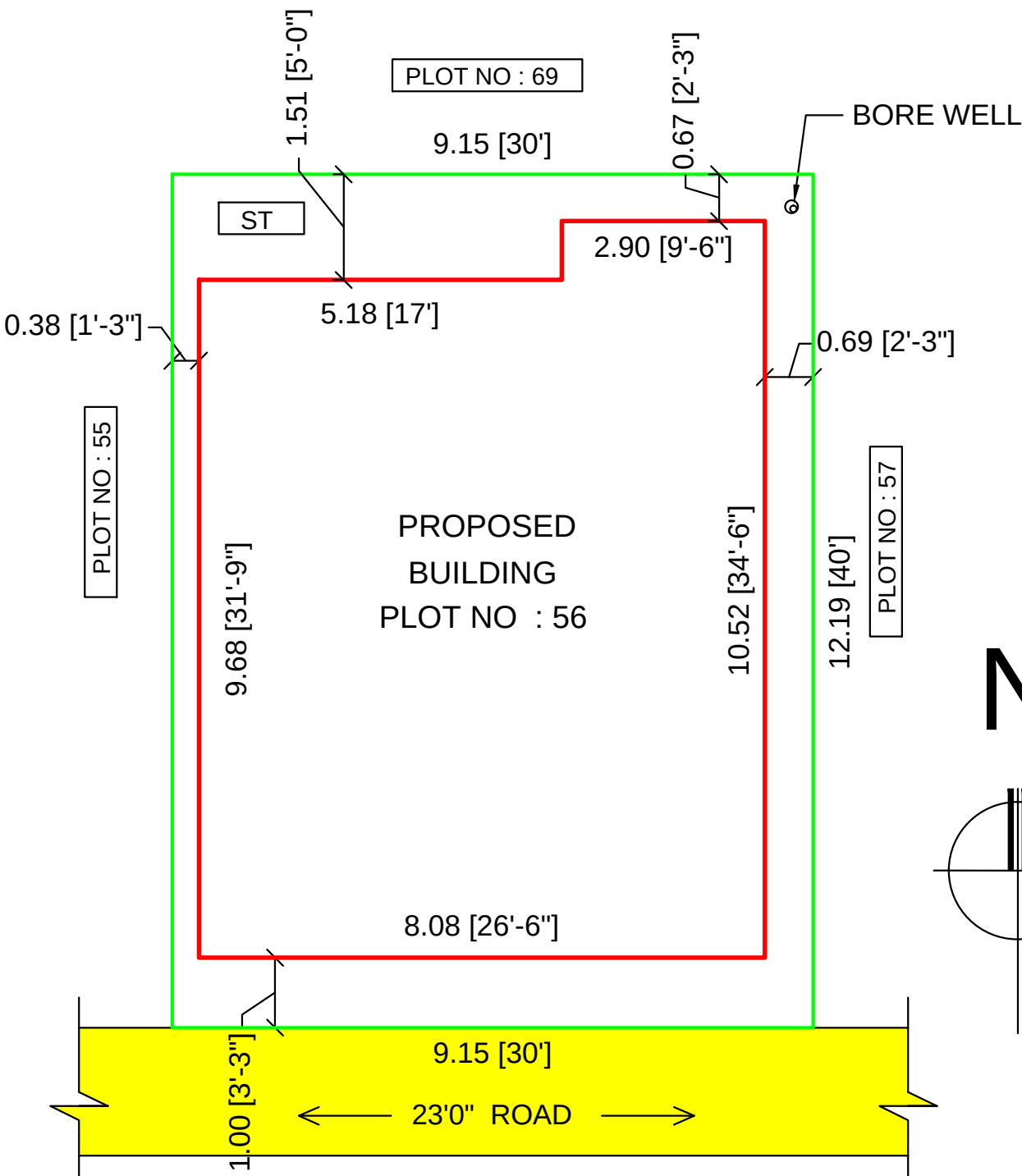
SITE PLAN
