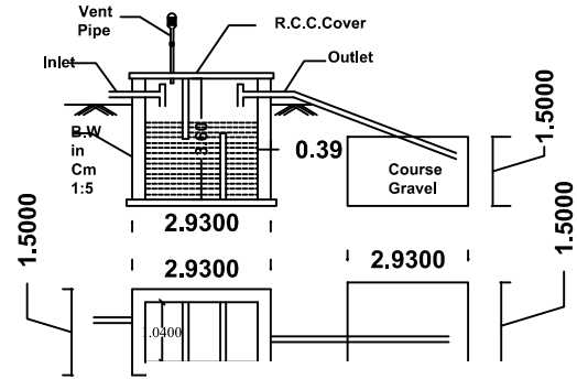
SEPTIC T
