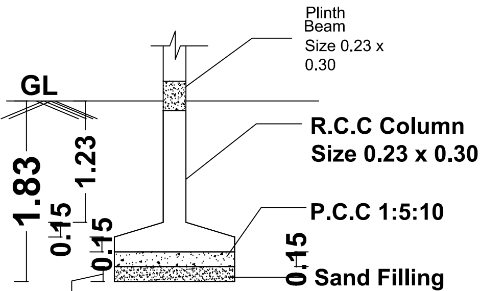
FOUNDATION DETAILS
