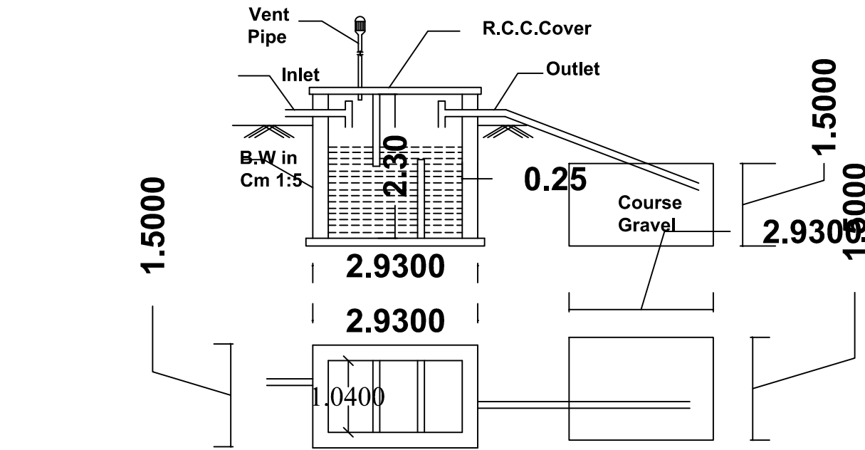
C TANK & D-TRENCH DETAILS
