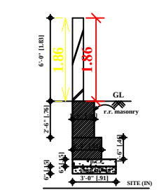
COMPOUND WALL
