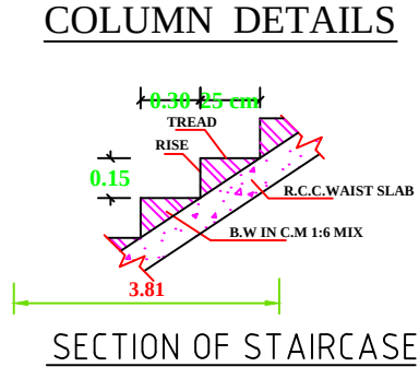
SECTION OF STAIRCASE
