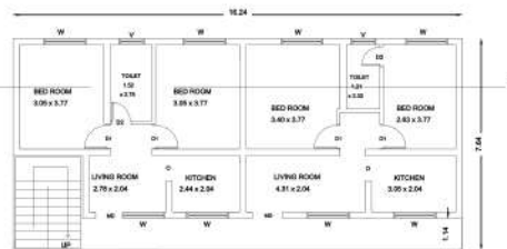
PRO. FIRST FLOOR PLAN
