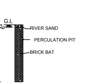
PERCUATION PIT
