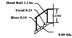
STAIRCASE DETAILS
