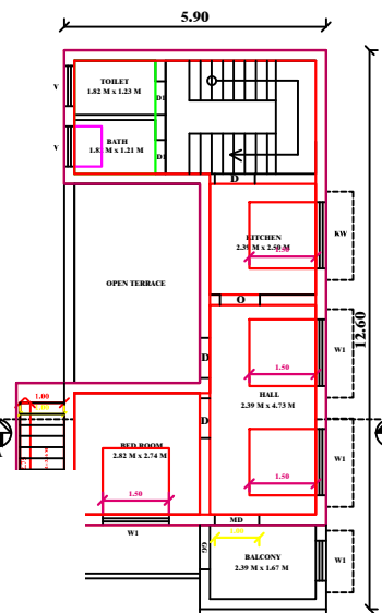
PROPOSED SECOND FLOOR PLAN
