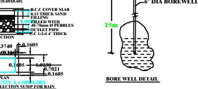
BORE WELL DETAIL
