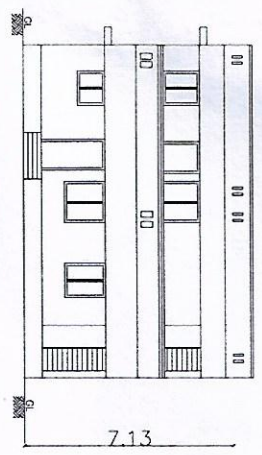
FRONT ELEVATION
