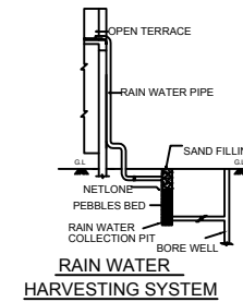
HARVESTING SYSTEM
