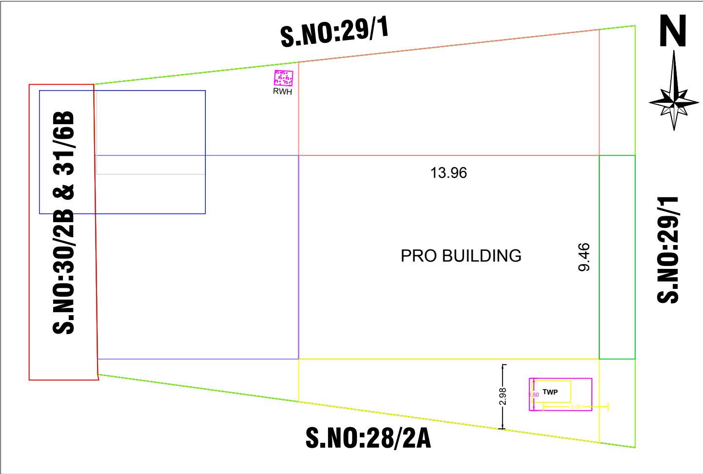
SITE PLAN
