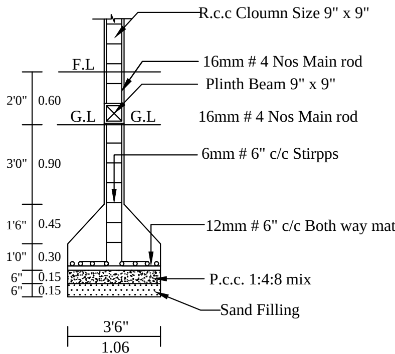
COLUMN DETAILS
