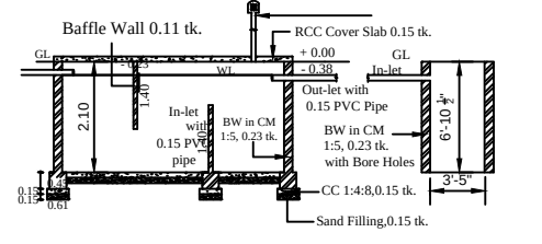
SECTION - SEPTIC TANK & SOAK PIT
