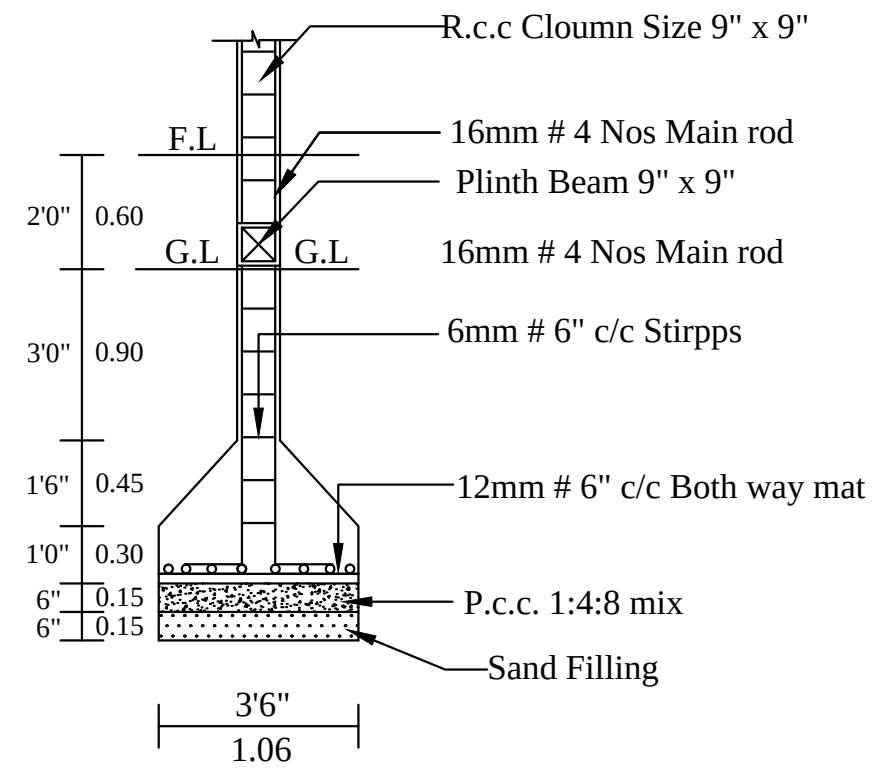
COLUMN DETAILS
