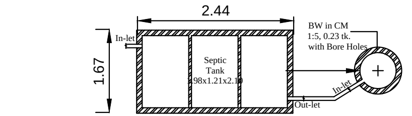
PLAN - SEPTIC TANK & SOAK PIT
