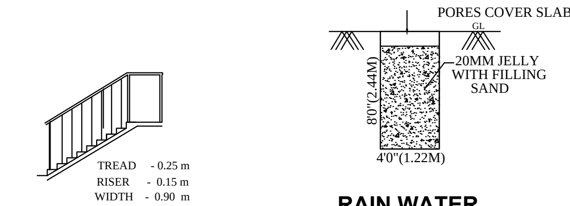
STAIRCASE DETAILS
