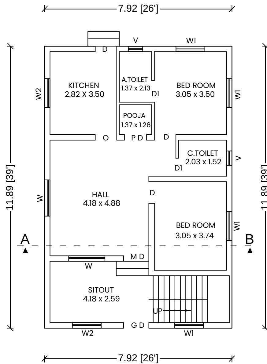
PLAN
