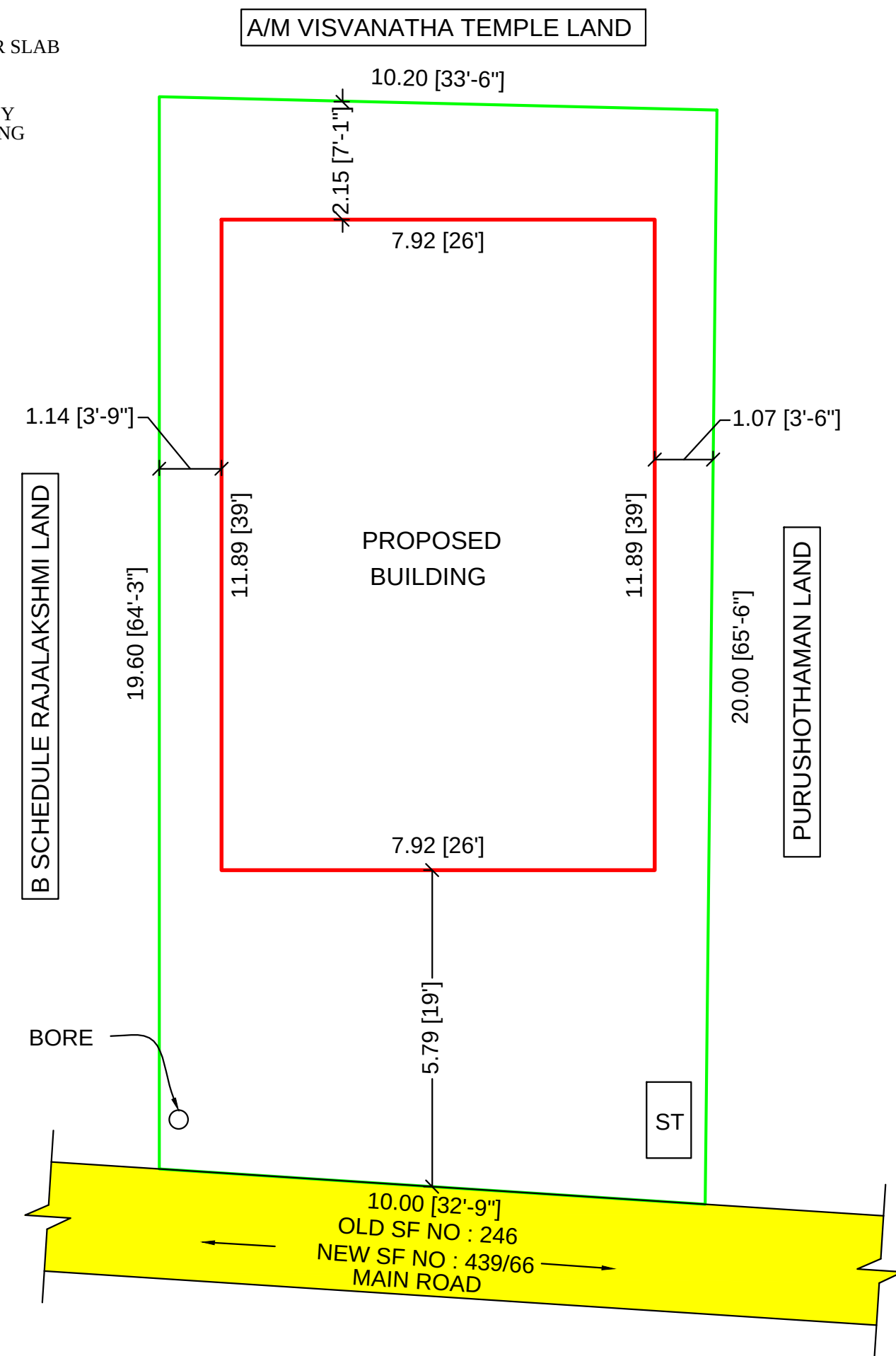
SITE PLAN
