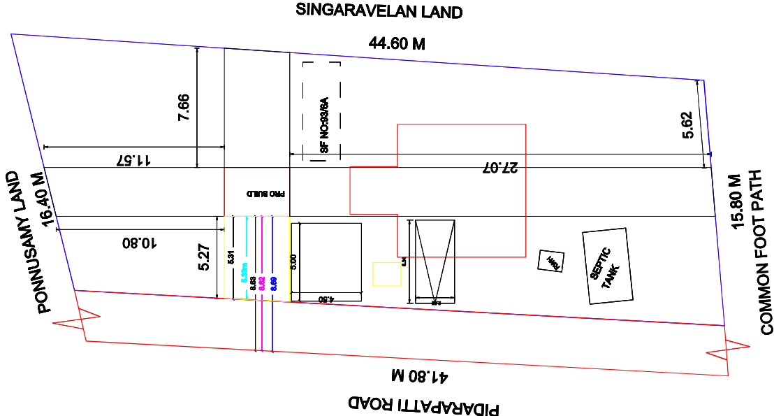
SITE PLAN (Not For Scale)
