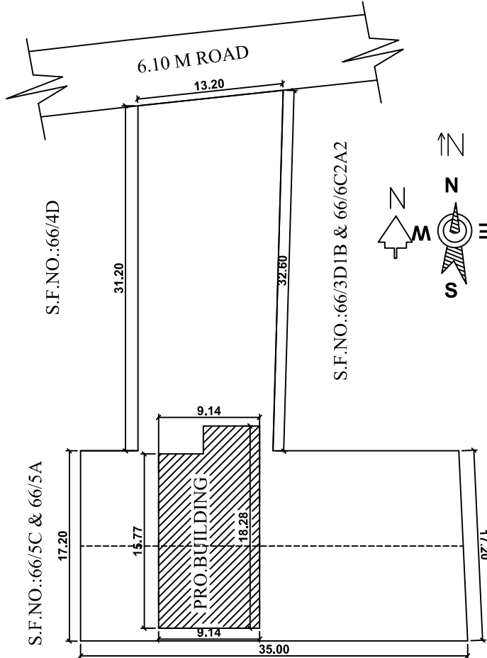
S.F.NO.:66/6C1B SITE PLAN (SCALE 1: 100)
