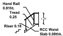
STAIRCASE DETAILS
