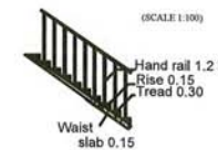
STAIRCASE
