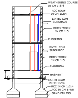
SECTION ON 'AB'
