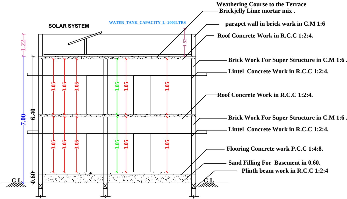
SECTION-AB
