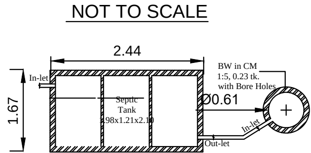
PLAN - SEPTIC TANK & SOAK PIT
