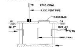
SEC. OF SEPTIC TANK
