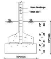
COLUMN FOUNDATION DETAIL
