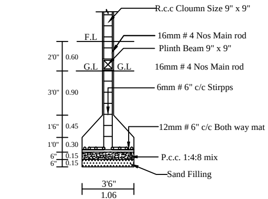
COLUMN DETIALS
