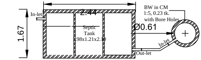
PLAN - SEPTIC TANK & SOAK PIT
