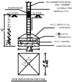
FOUNDATION DETAIL
