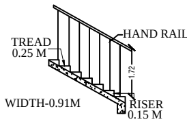
STAIRCASE DETAILS
