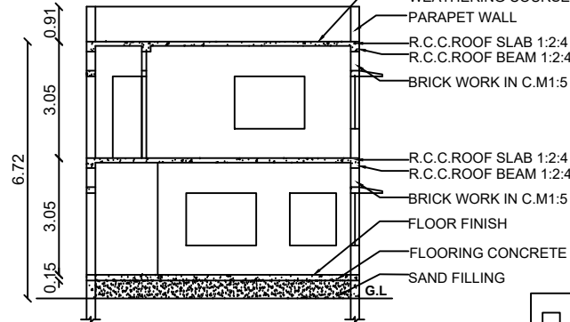
SECTION ON SS
