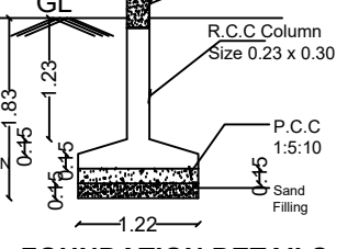
FOUNDATION DETAILS
