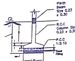
FOUNDATION DETAILS
