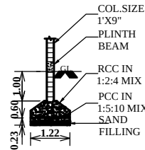
COLUMN DETAILS
