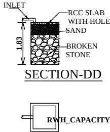
PLAN OF RWH
