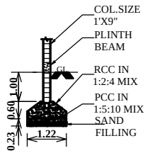
COLUMN DETAILS
