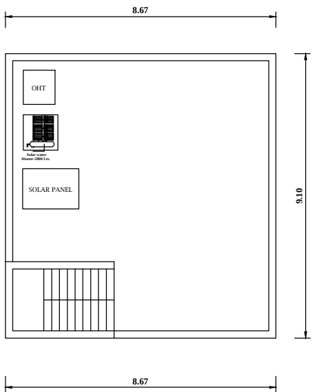
PRO GROUND FLOOR ROOF PLAN
