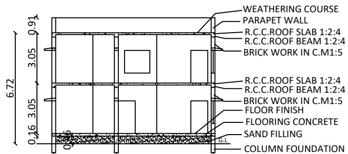
SECTION- SS
