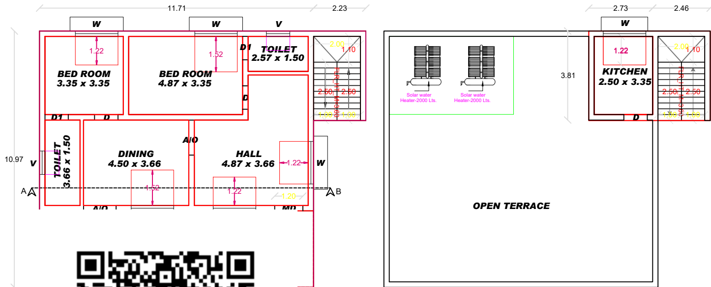
FIRST FLOOR PLAN OPEN TERRACE PLAN
