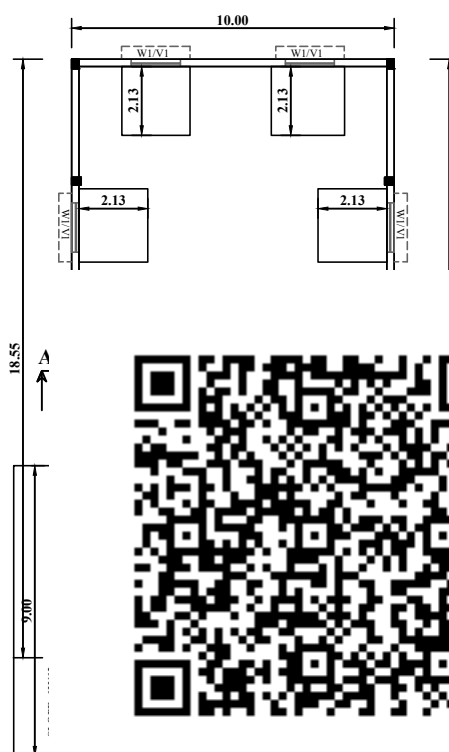
PROPOSED BUILDING PLAN
