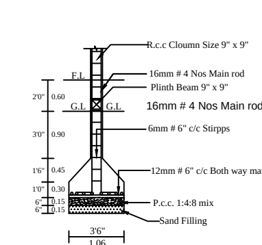
COLUMN DETIAL
