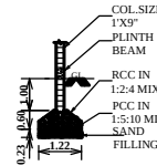
COLUMN DETAILS
