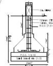
R.C.C. COLUMN FOOTING DETAILS SCALE: 1:20
