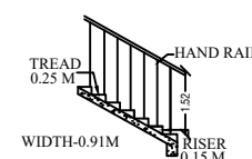
STAIRCASE DETAILS
