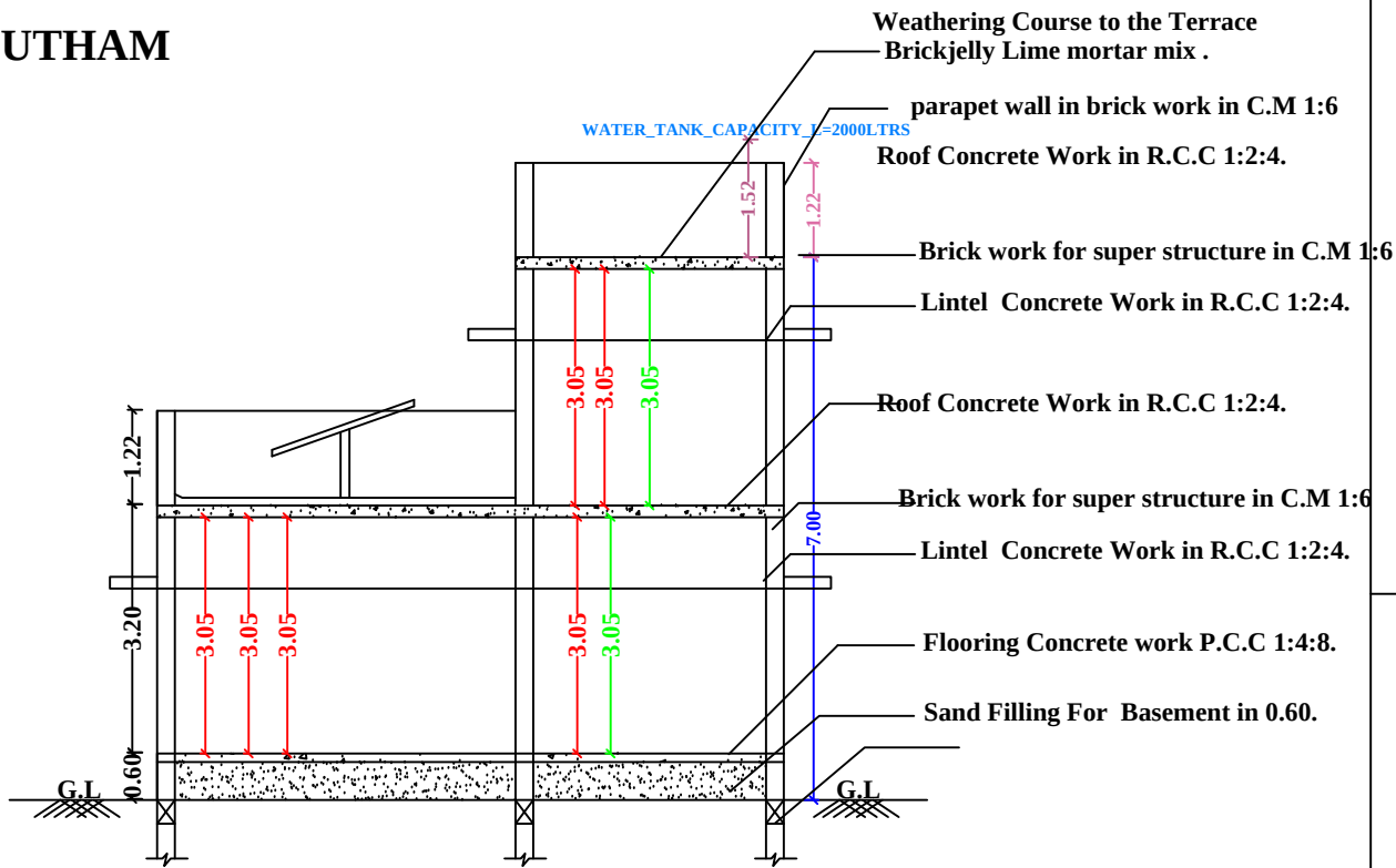
SECTION-AB
