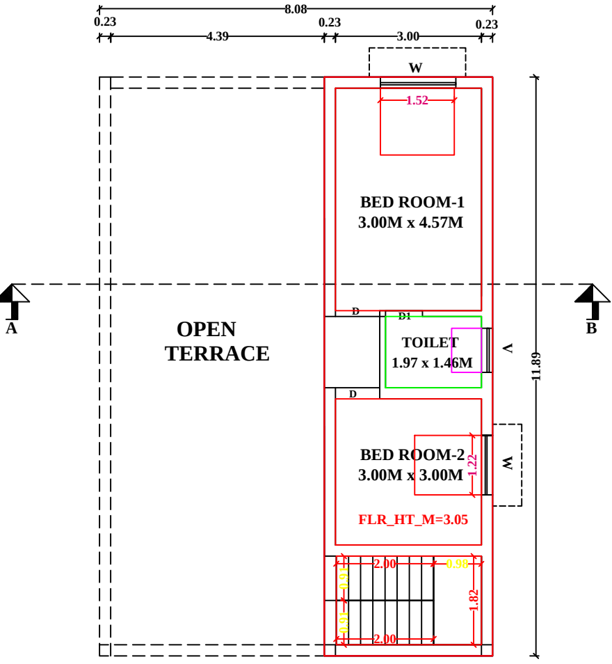
FLOOR-01 PRO.FIRST FLOOR PLAN
