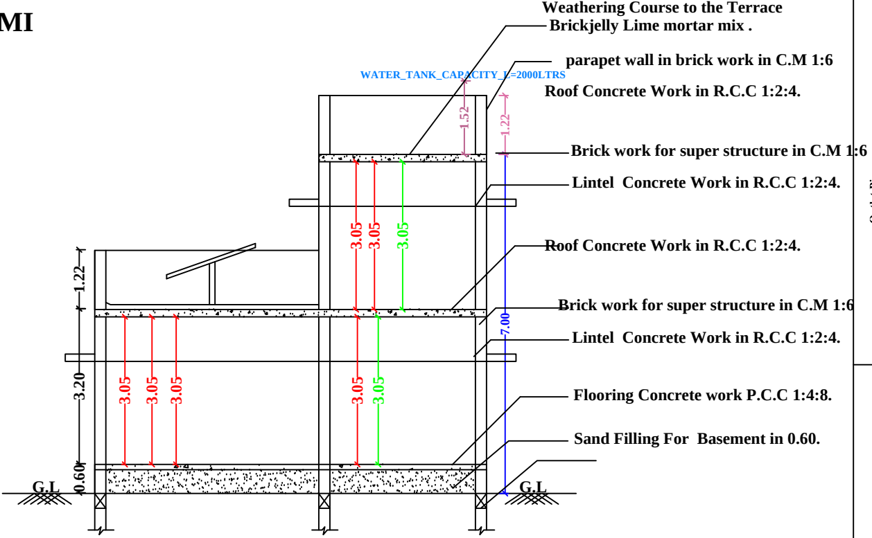
SECTION-AB
