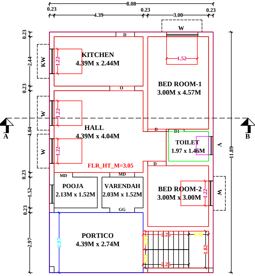
FLOOR-GROUND PRO.GROUND FLOOR PLAN
