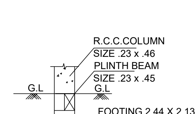
FOUNDATION DETAIL-B
