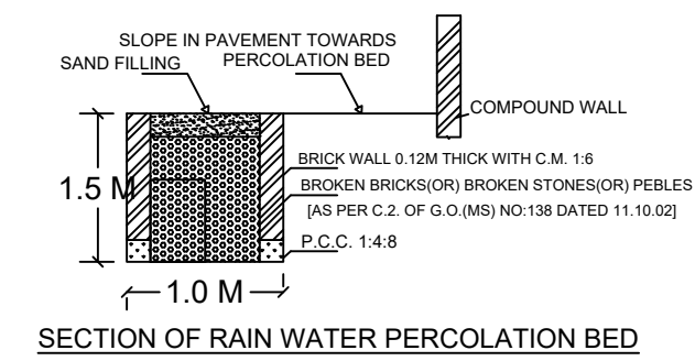
SECTION OF RAIN WATER PERCOLATION BED
