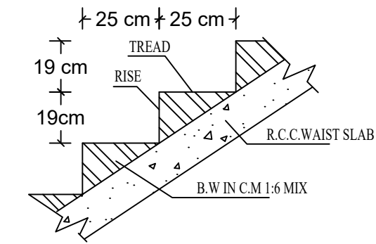
SECTION OF STAIRCASE
