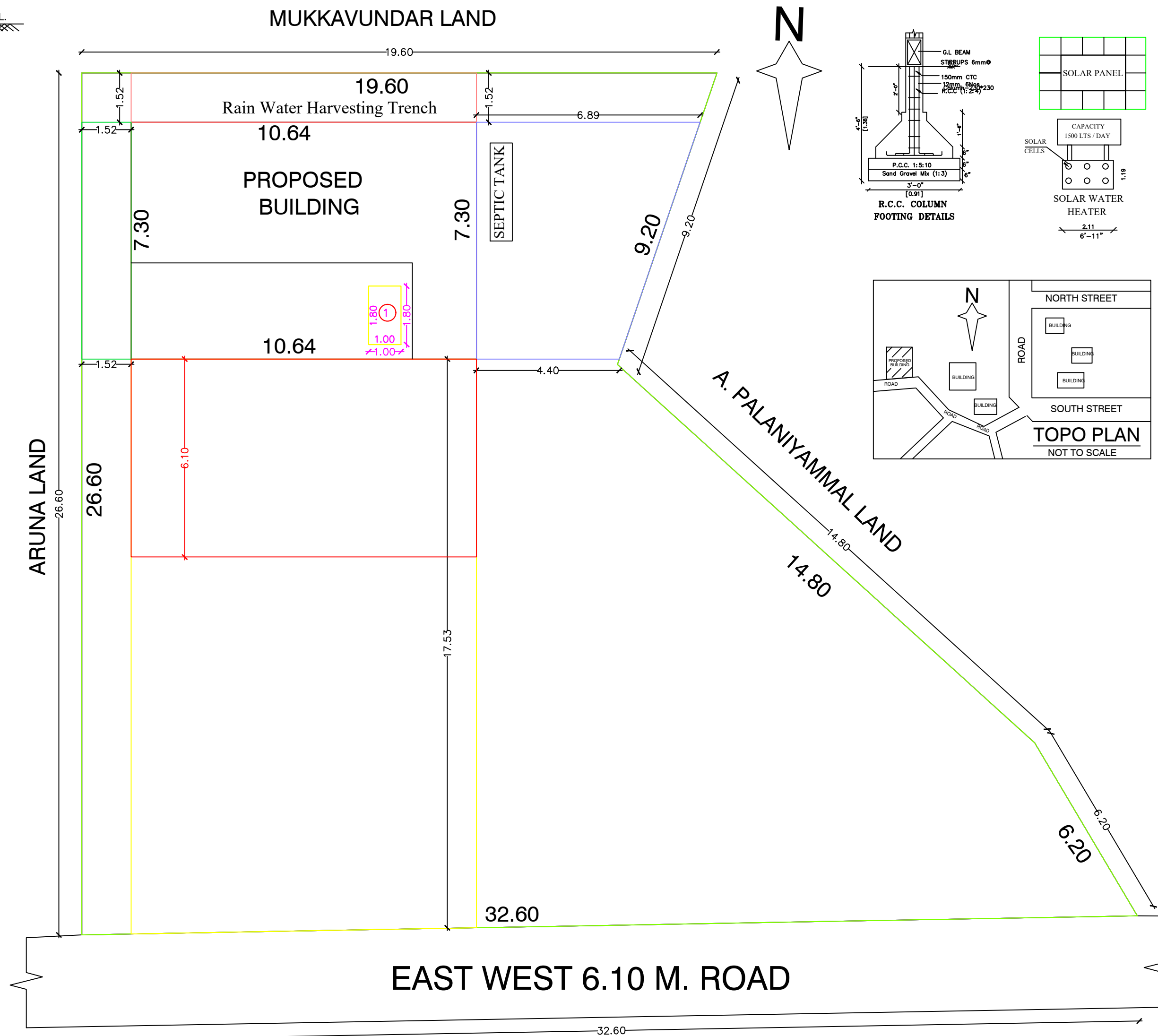
SITE PLAN
