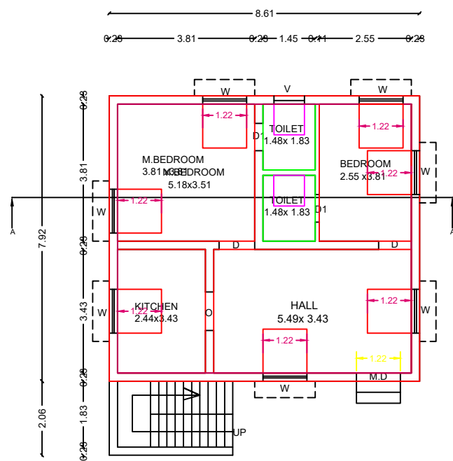
FLOOR PLAN
