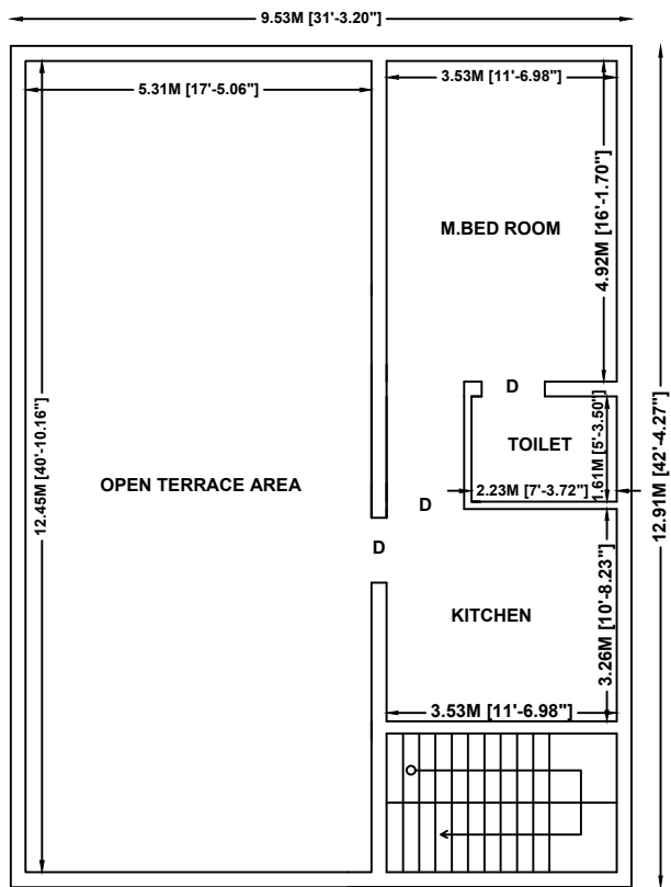
PROPOSED FRIST FLOOR PLAN
