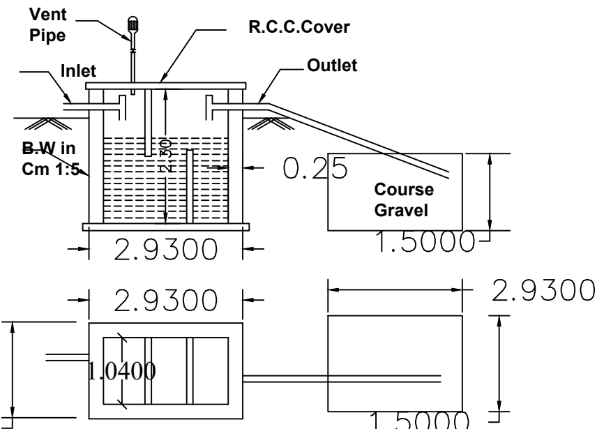
SEPTIC TANK & D-TRENCH DETAILS
