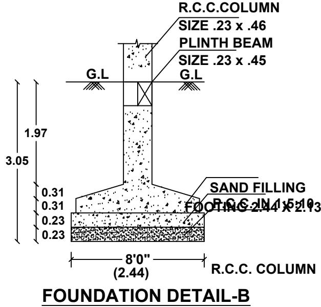
FOUNDATION DETAIL-B
