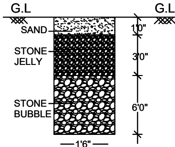
RAIN WATER HARVEST PIT (RWHP)
