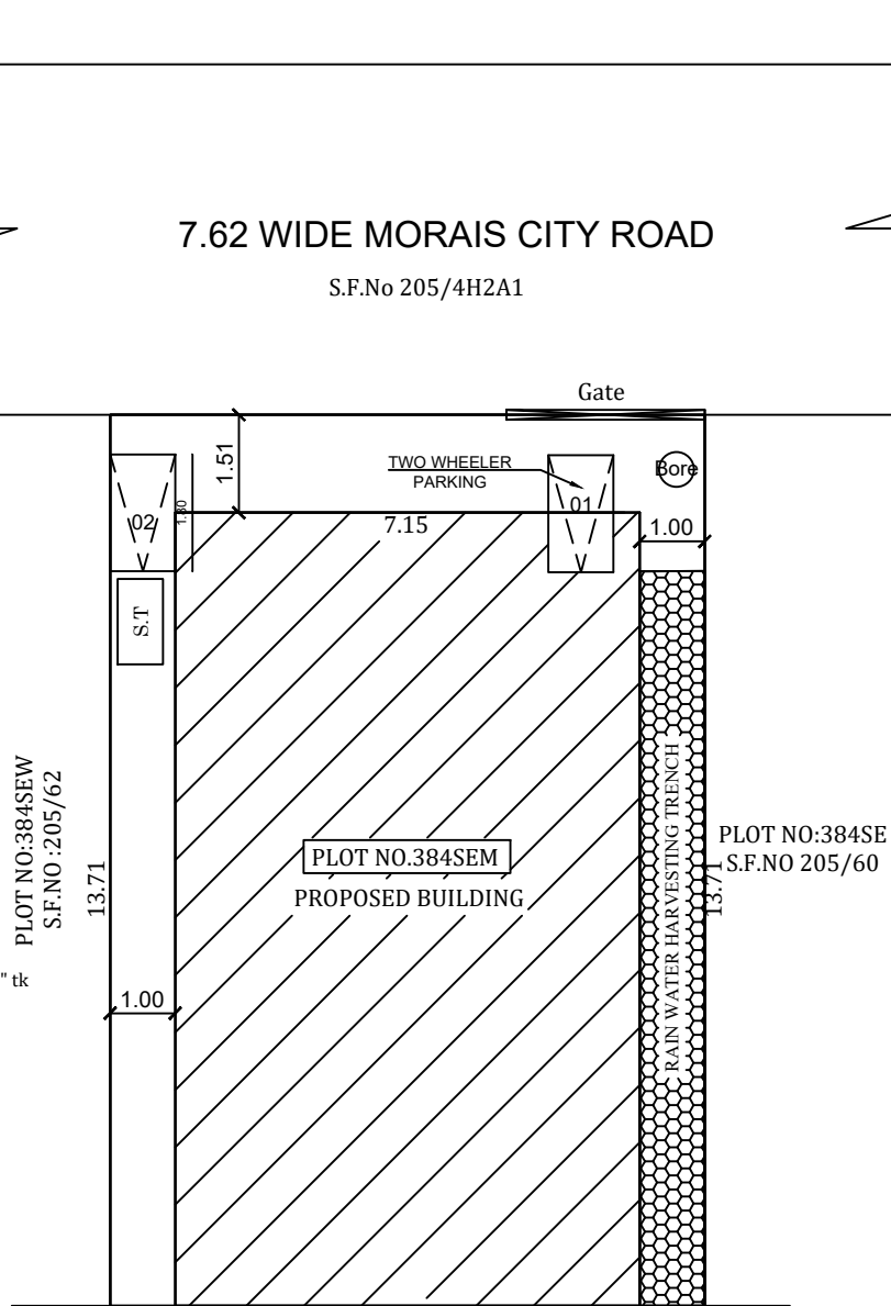
PLOT NO:384SEM S.F.NO:205/62 PROPOSED BUILDING SCALE 1:100
