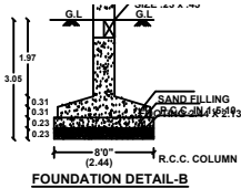
FOUNDATION DETAIL-B
