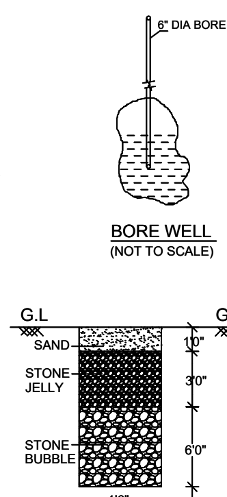
RAIN WATER HARVEST PIT (RWHP)
